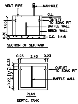
SEPTIC TANK:-
