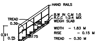
STAIRCASE DETAILS:-
