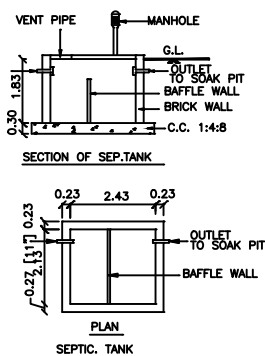
SEPTIC TANK:-
