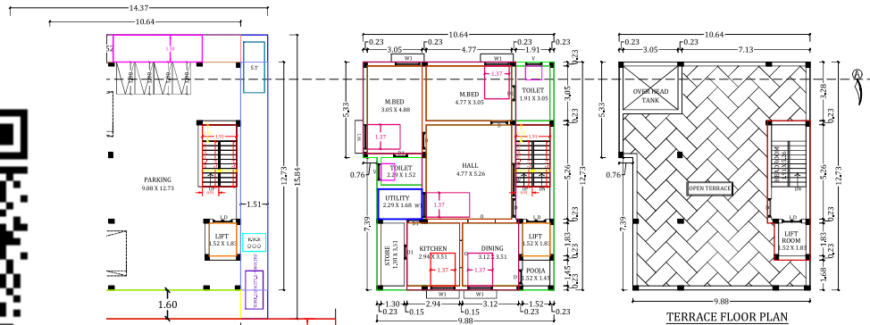
TYPICAL FLOOR PLAN FIRST, SECOND & THIRD FLOOR PLAN TYPICAL_FLOOR_PLAN=1,2,3
