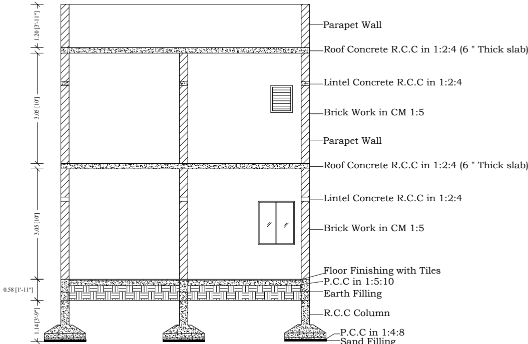
SECTION X-X
