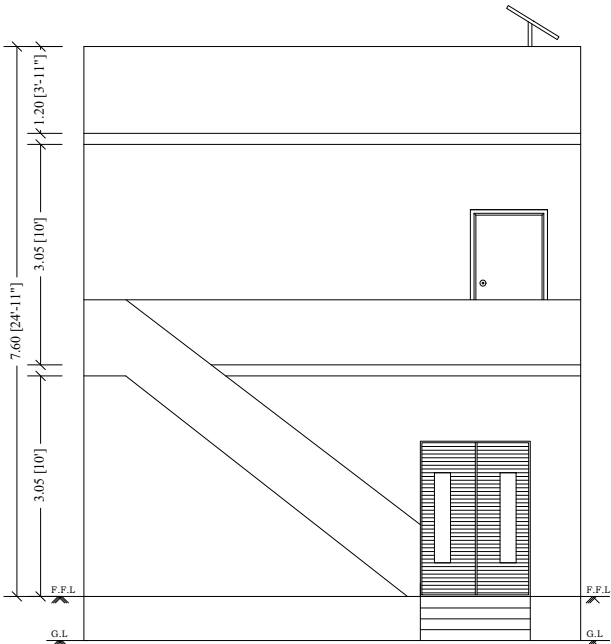
FRONT ELEVATION
