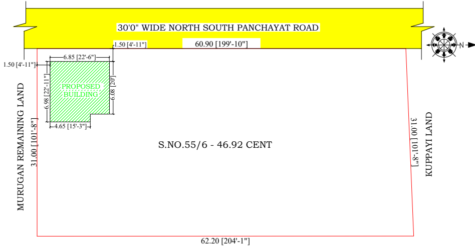
SITE PLAN (SCALE -1:250)
