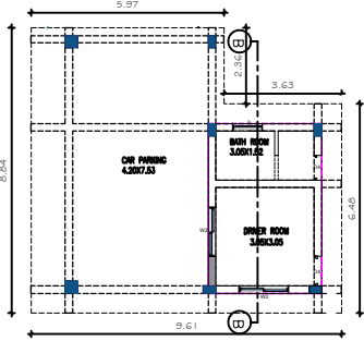
PROPOSED OF GROUND FLOOR PLAN (BLOCK-02)
