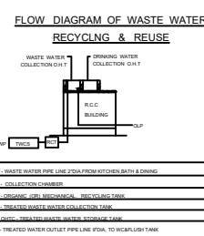
FLOW DIAGRAM OF WASTE WATER RECYCLING & REUSE
