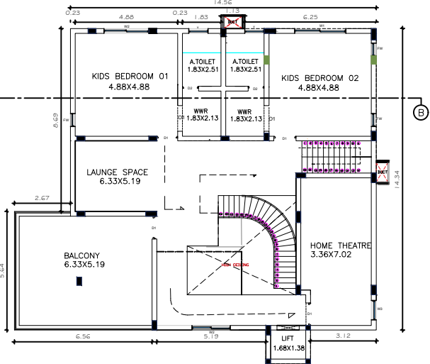
PROPOSED OF FIRST FLOOR PLAN
