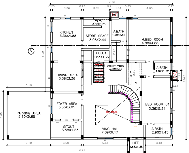
PROPOSED OF GROUND FLOOR PLAN
