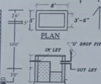
SEPTICTANK DETAILS
