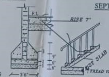
STAIRCASE DETAILS
