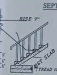
STAIRCASE DETAILS
