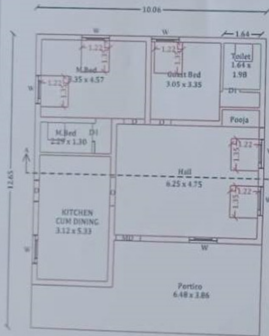
PRO.GROUND FLOOR
