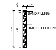
DETAILS OF PERCOLATION PIT
