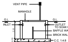
SECTION OF SEP. TANK
