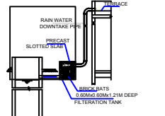
RAIN WATER HARVESTING SYSTEM
