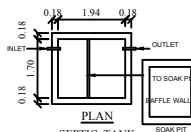
PLAN SEPTIC TANK
