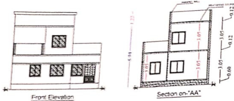
Front Elevation
