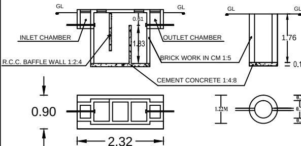
DETAILS OF SEPTIC TANK & SOAK PIT.
