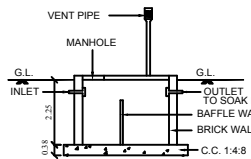
SECTION OF SEPT. TANK
