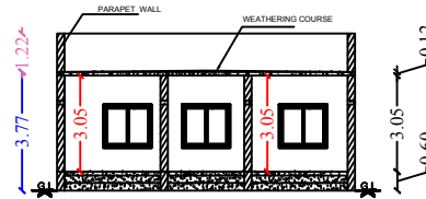
Section on-"AA"
