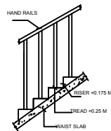
STAIR CASE DETAILS
