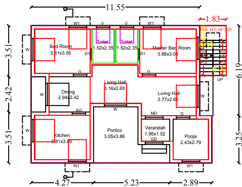
Ground Floor
