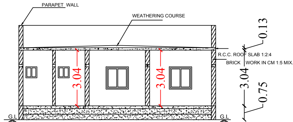
Section on-"AA"
