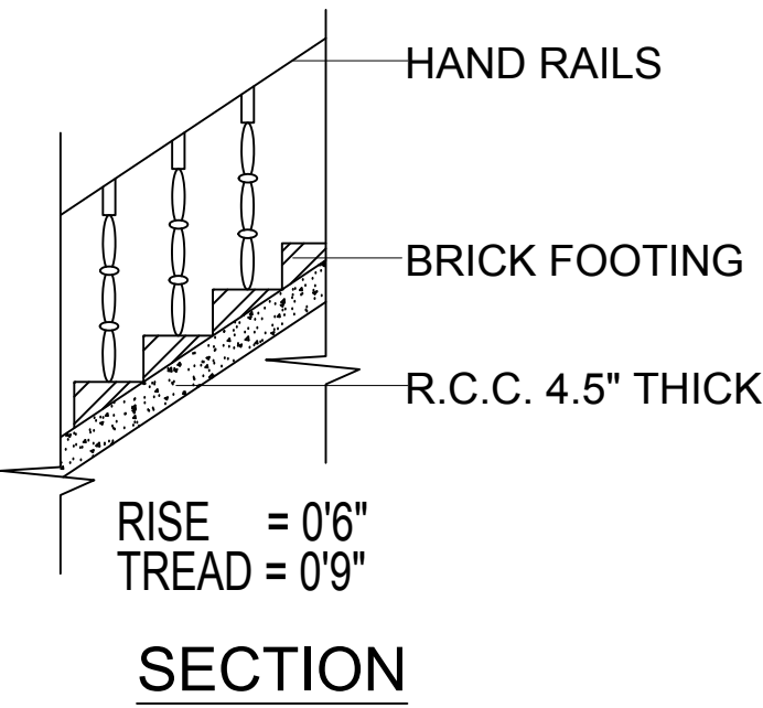
SECTION
