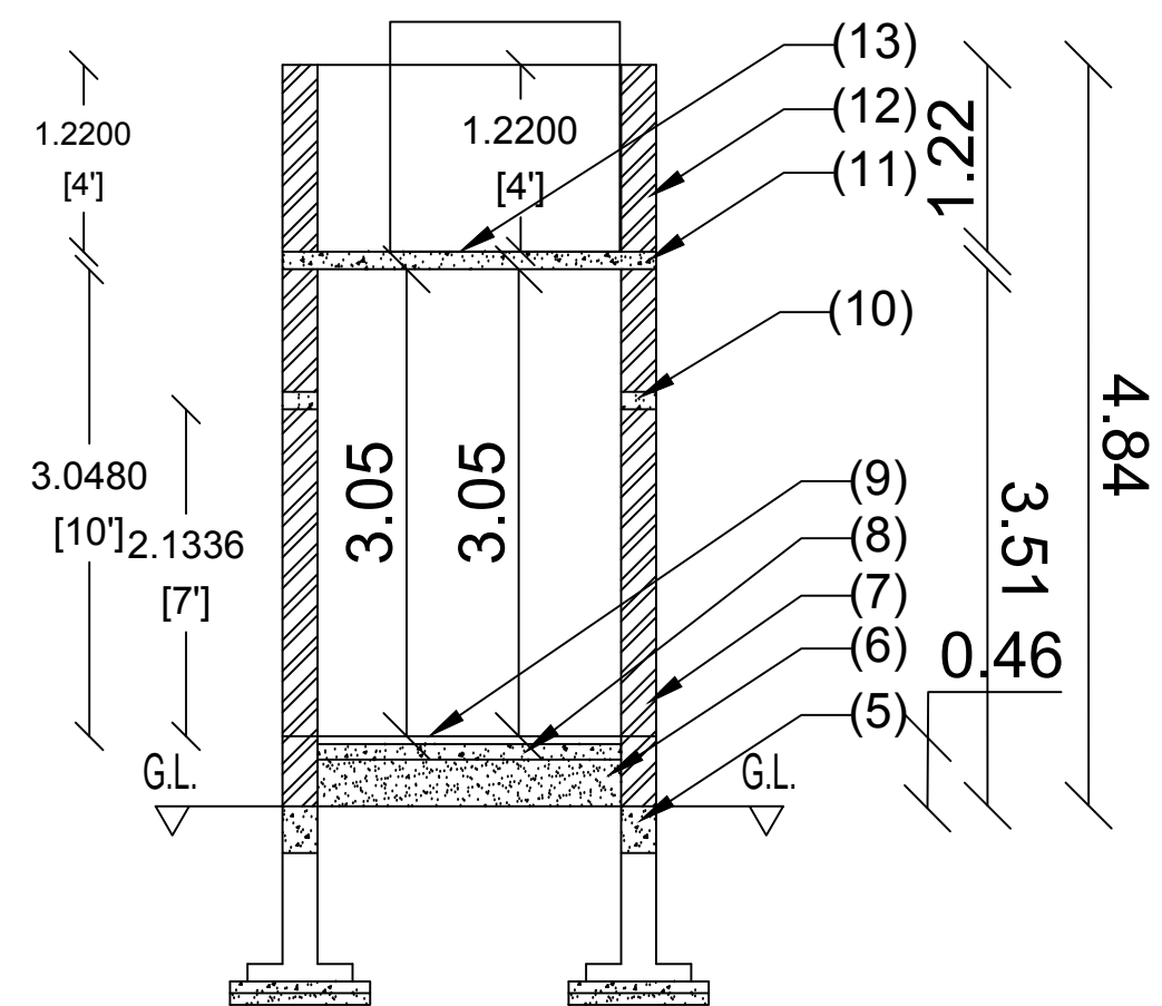
SECTION "AA"
