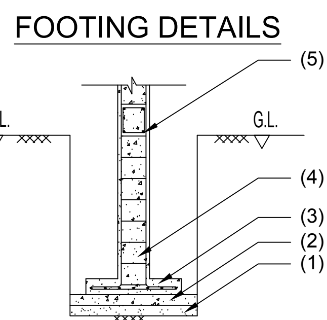
SECTION
