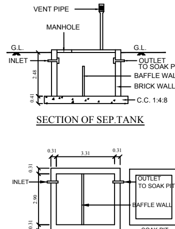
PLAN SEP. TANK
