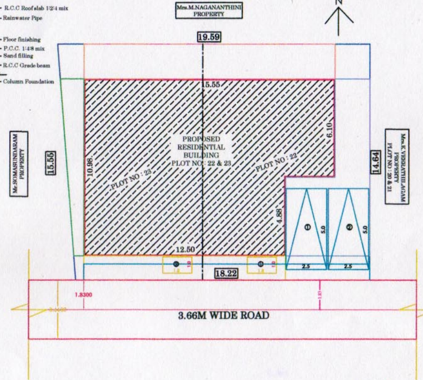
SITE PLAN
