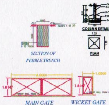
MAIN GATE
