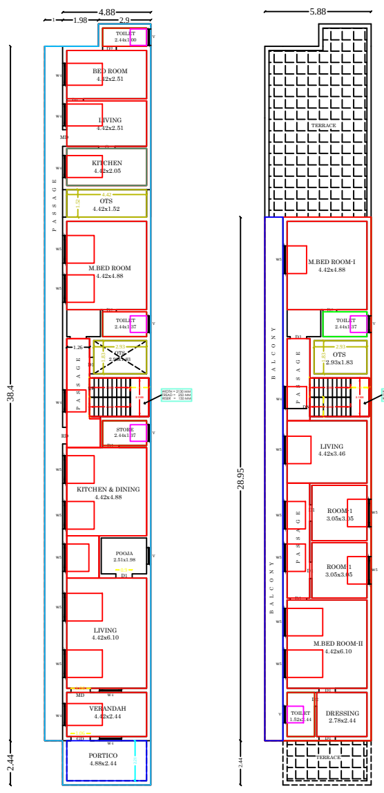
PROPOSED BUILDING FLOOR - 0 GROUND FLOOR PLAN PROPOSED BUILDING FLOOR - 01 FIRST FLOOR PLAN
