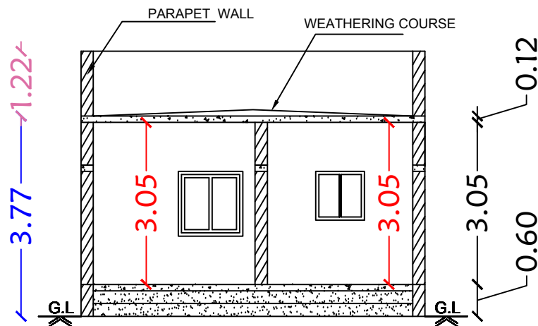
Section on-"AA"
