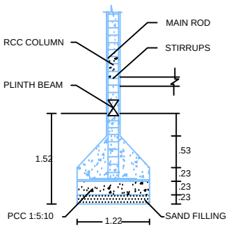
COLUMN DETAILS
