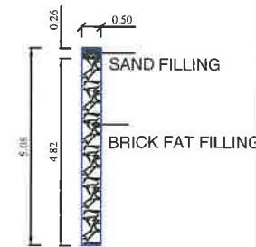
DETAILS OF PERCOLATION PIT
