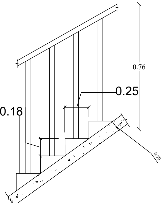
SECTION OF STAIRCASE
