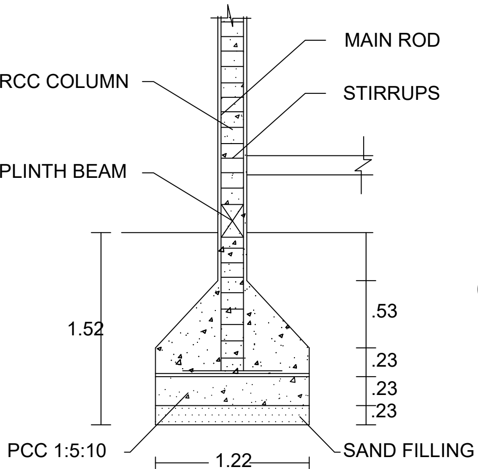
COLUMN DETAILS
