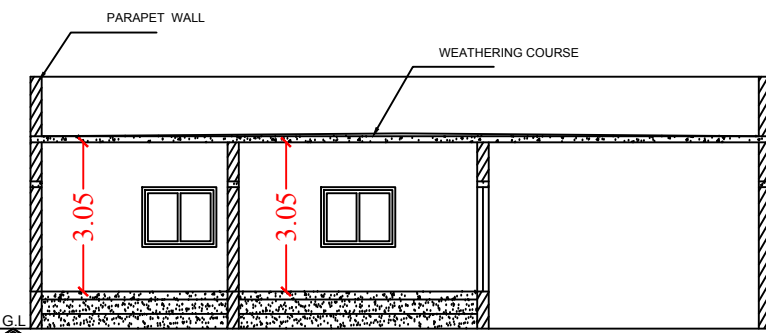
Section on-"AA"
