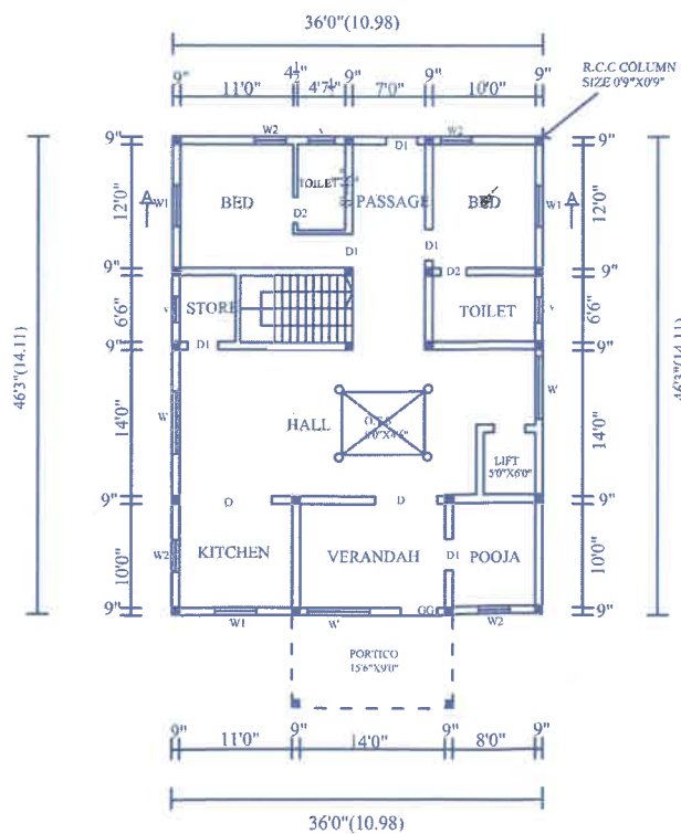
PLAN OF GROUND FLOOR
