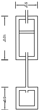
PLAN OF SEPTIC TANK/
