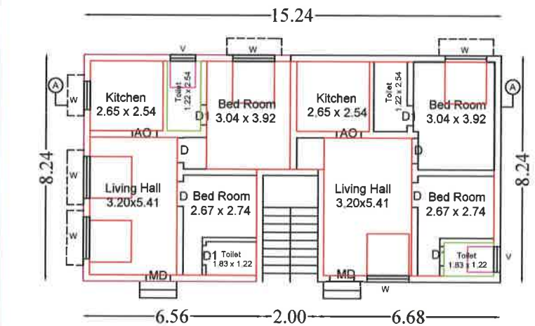
Floor - Ground
