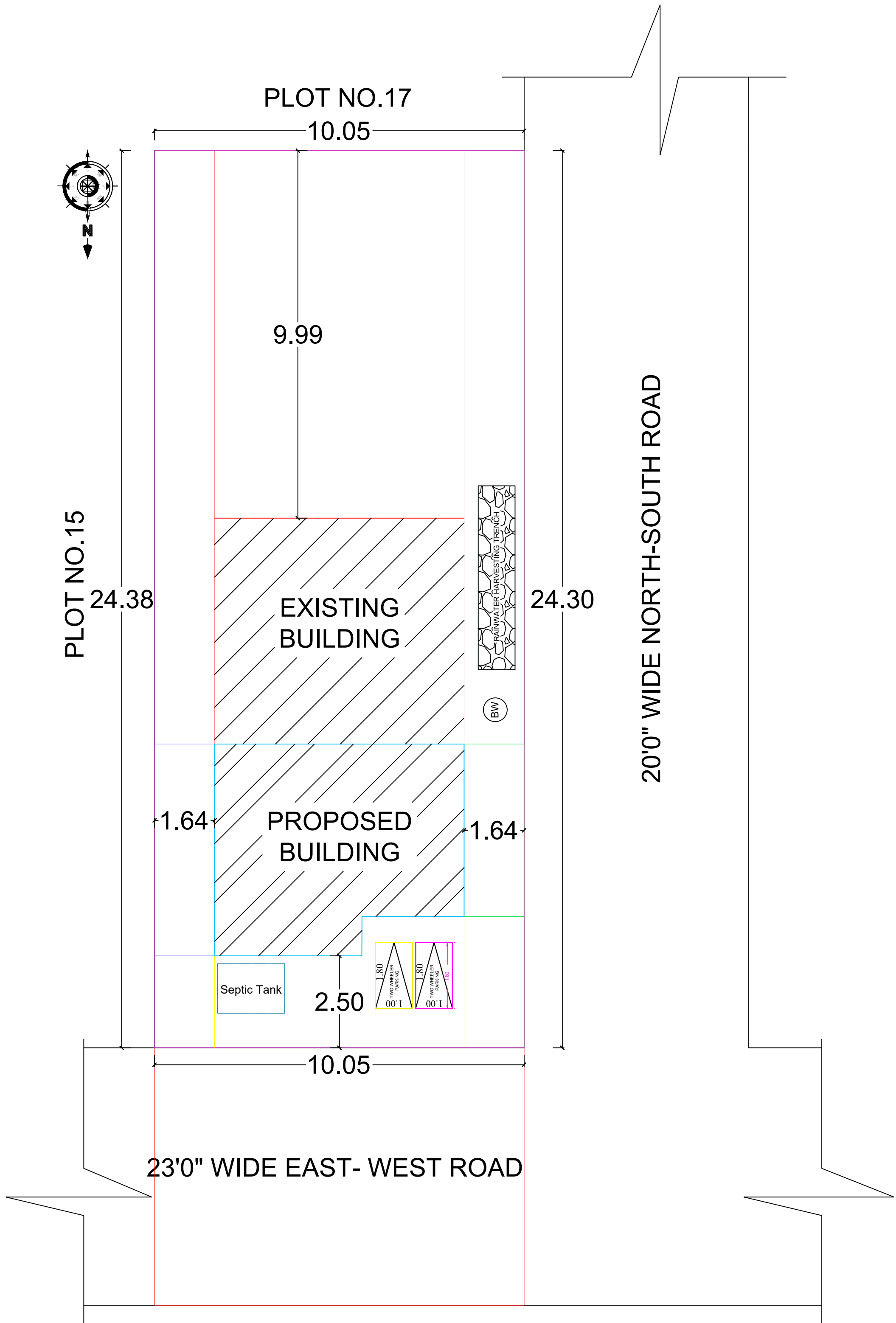
SITE PLAN (1:100)
