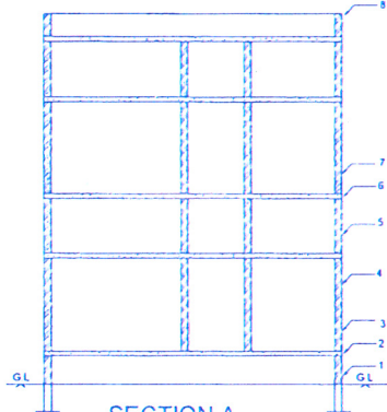
SECTION A
