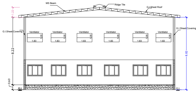
Section on-"AA"
