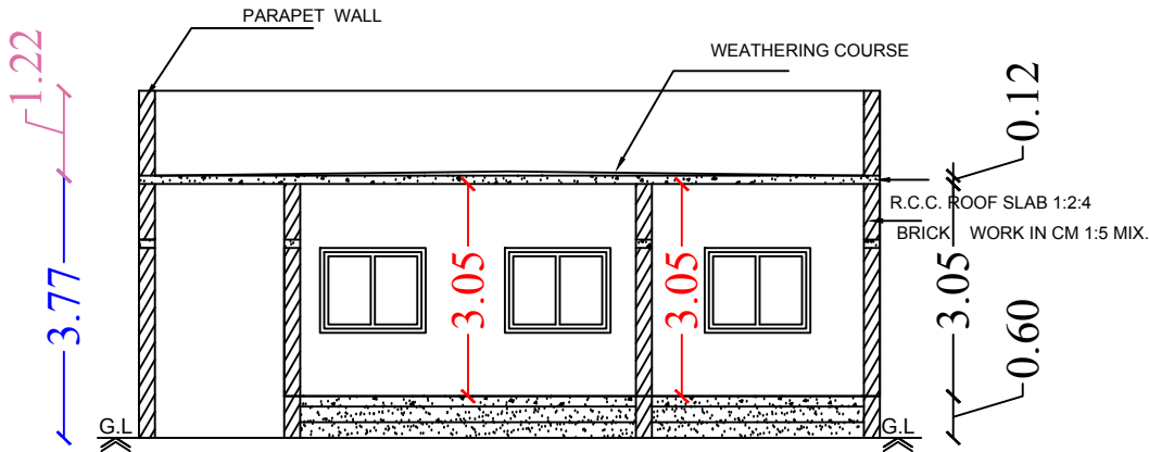
Section on-"AA"
