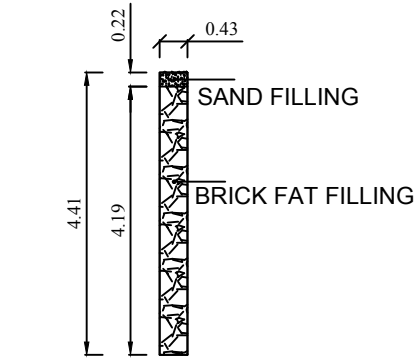
DETAILS OF PERCULATION PIT
