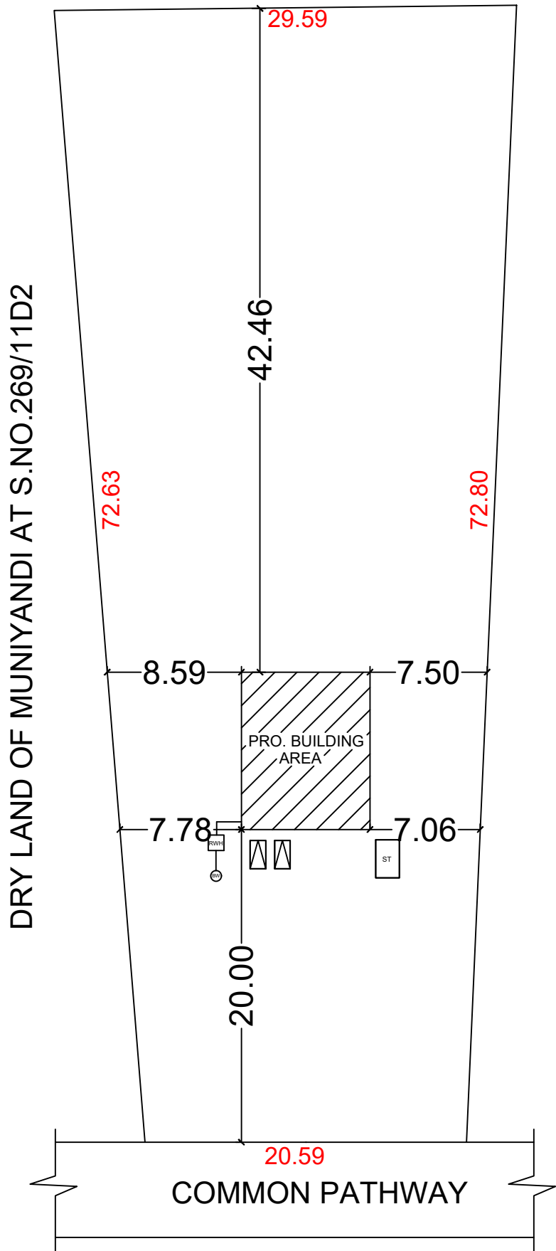
SITE PLAN
