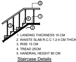
Staircase Details
