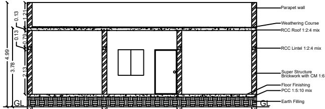
SECTION ON "VR"
