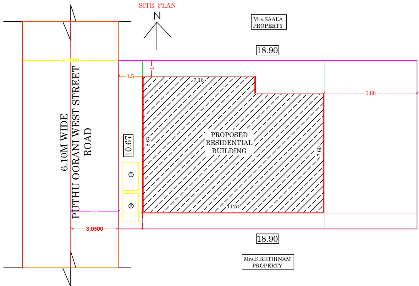
SITE PLAN
