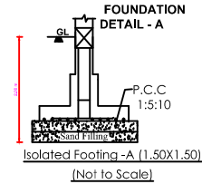
Isolated Footing - A (1.50X1.50)
