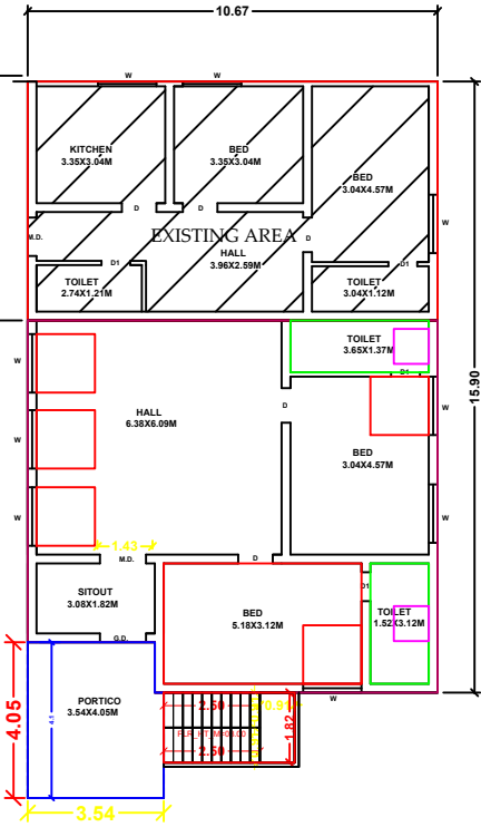
EXISTING &PROPOSED GROUND FLOOR PLAN
