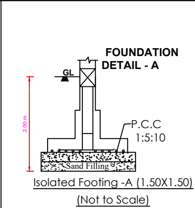
Isolated Footing -A (1.50X1.50) (Not to Scale)
