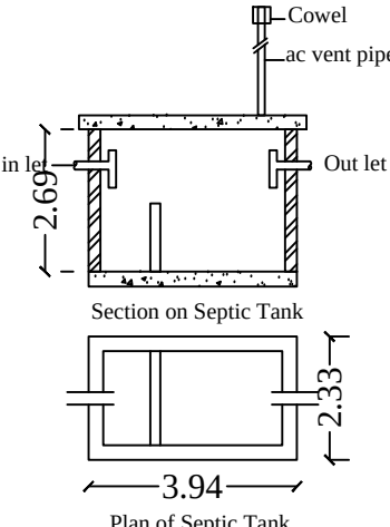
Plan of Septic Tank
