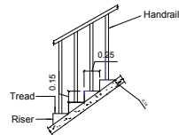
STAIRCASE DETAIL
