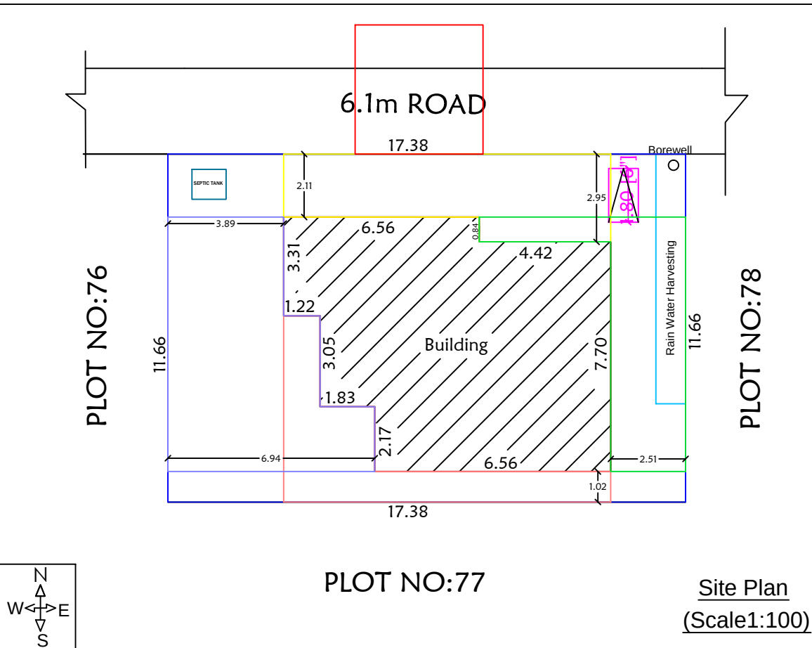
RAIN WATER HARVESTING SYSTEM
