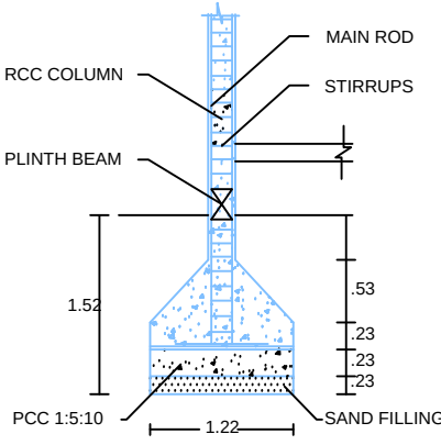
COLUMN DETAILS
