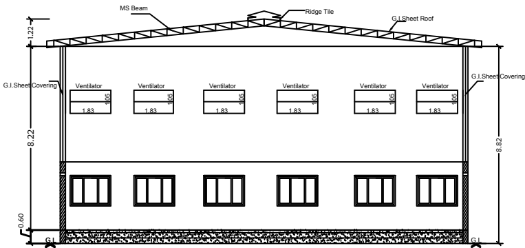
Section on-"AA"
