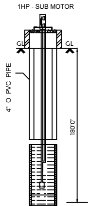
Bore Well Details
