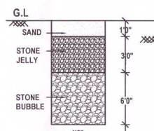
RAIN WATER HARVEST PIT (RWHP)
