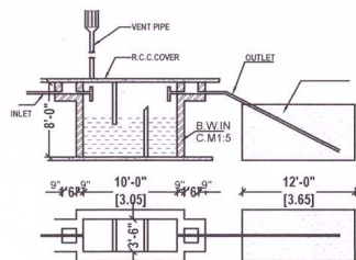
SEPTIC TANK & D-TRENCH DETAILS (NOT TO SCALE)
