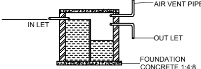
SEPTIC TANK DETAILS
