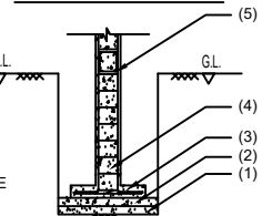
FOOTING DETAILS
