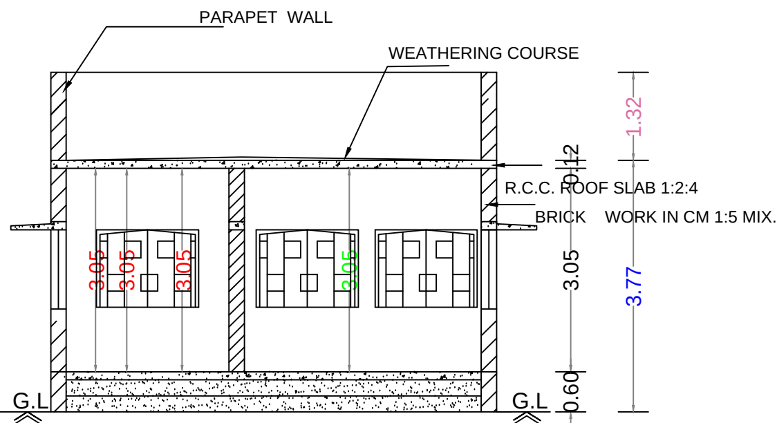
Section on-"AA"
