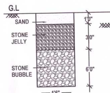
RAIN WATER HARVEST PIT (RWHP)
