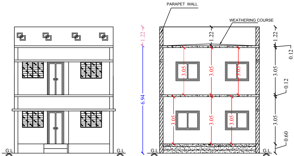
Section on-"AA"
