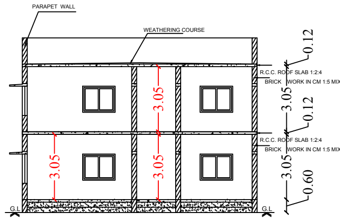
Section on-"AA"
