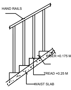
STAIR CASE DETAILS
