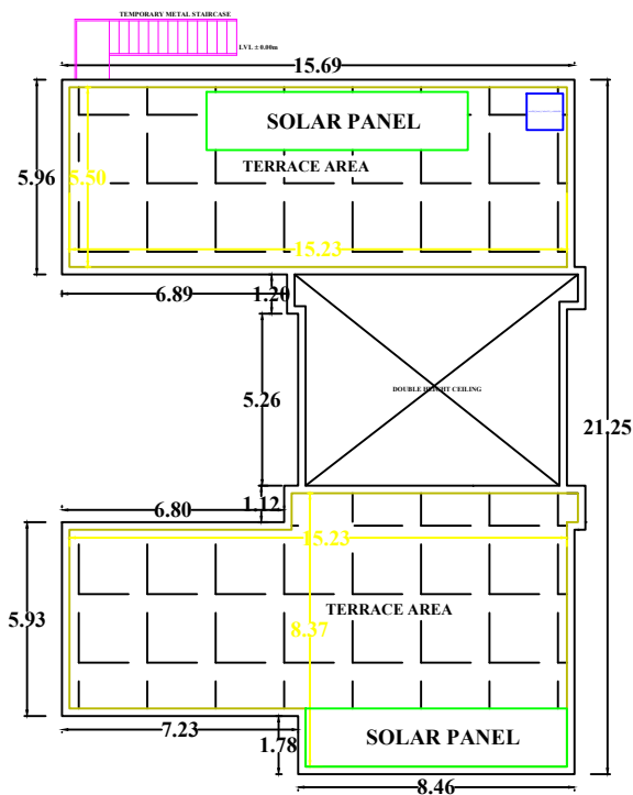
PRO.TERRACE FLOOR PLAN
