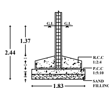
COLUMN DETAILS [NOT TO SCALE]
