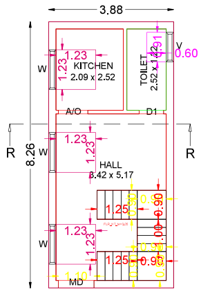
Pro.Ground Floor Plan
