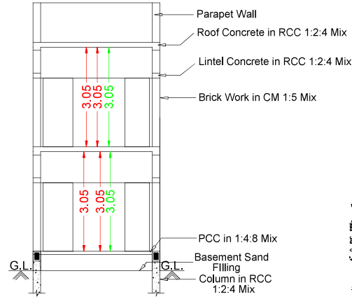
Section RR
