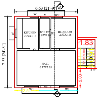
EXISTING GROUND FLOOR PLAN
