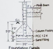
Foundation Details
