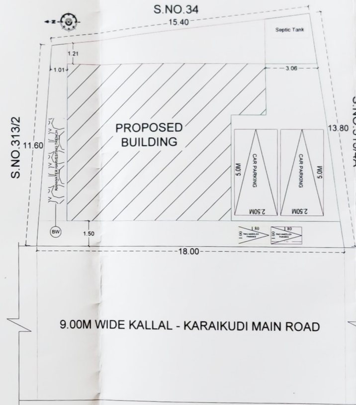
SITE PLAN (1:100)
