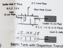
Septic Tank with Dispersion Trench
