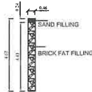
DETAILS OF PERCOLATION PIT
