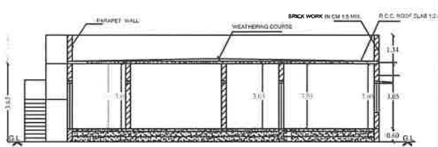
Section on-AA
