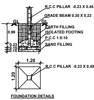
FOUNDATION DETAILS
