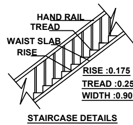
STAIRCASE DETAILS
