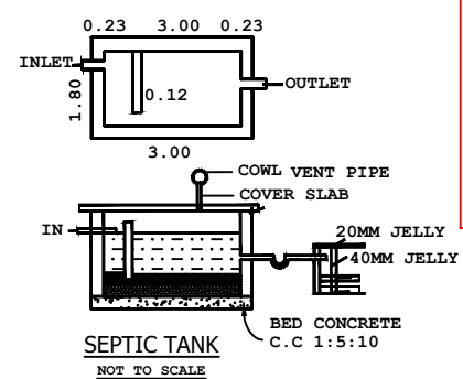
SEPTIC TANK
