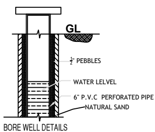
BORE WELL DETAILS
