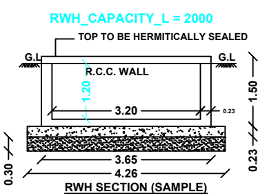
RW SECTION (SAMPLE)
