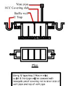
Septic Tank With U-Trap Not To Scale
