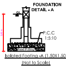
Foundation Detail - A Isolated Footing - 24" (1.50' X 1.50') Not To Scale
